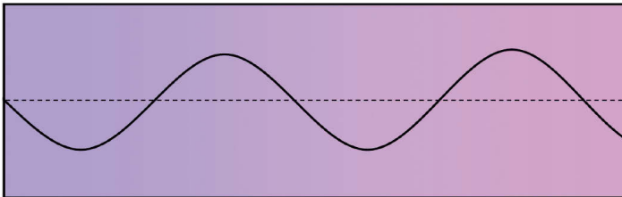
Figure 36.2 Different pseudofrequencies.
