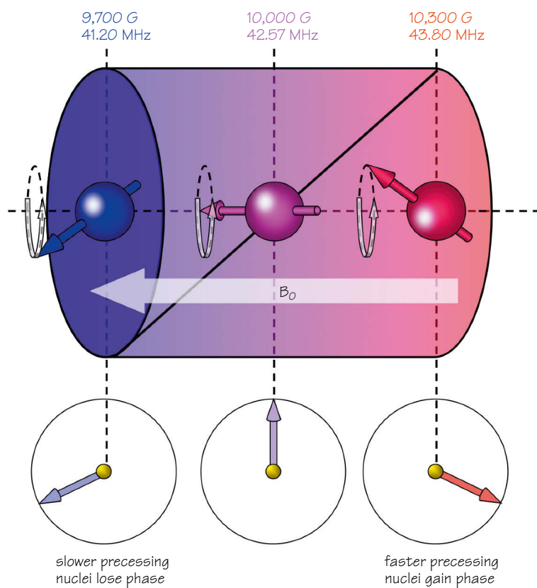
Figure 29.1 Phase encoding.
