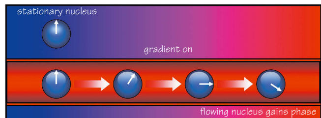
Figure 50.4 Intravoxel dephasing.
