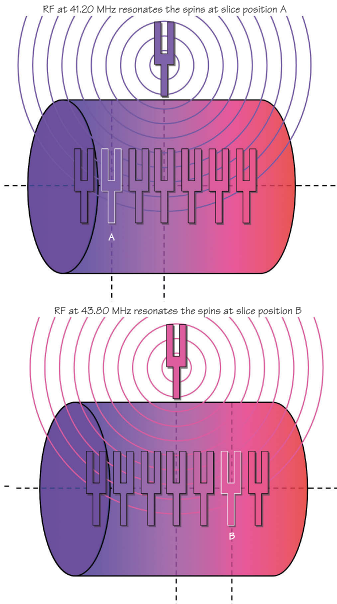
Figure 28.1 Slice selection.
