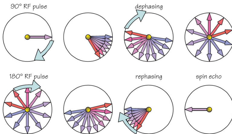
Figure 13.1 180^\circ RF rephasing.
