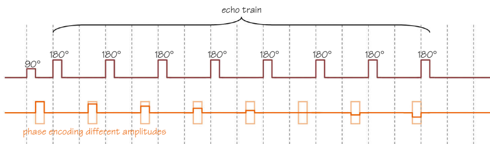
Figure 14.1 The echo train in TSE.
