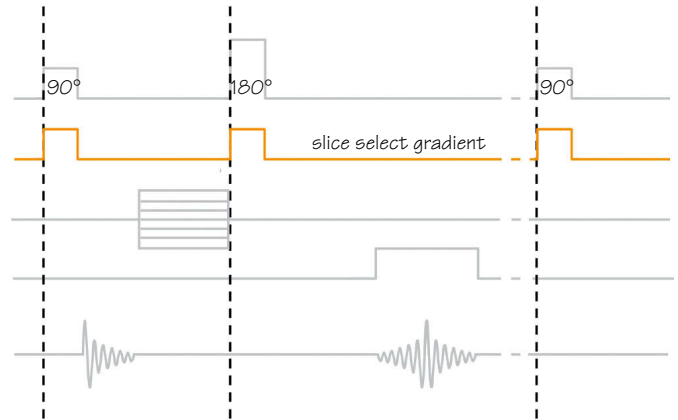
Figure 28.3 Timing of slice selection in a spin-echo pulse sequence.
