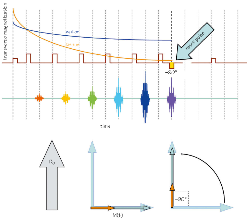
Figure 15.3 The fast recovery or 'drive' sequence.
