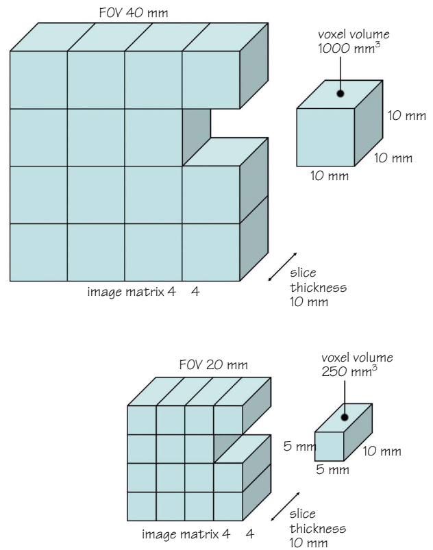
Figure 42.2 FOV versus SNR and resolution.
