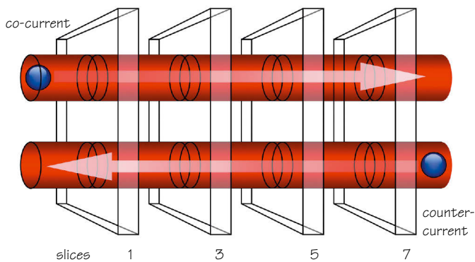
Figure 50.3 Co- and counter-current flow.
