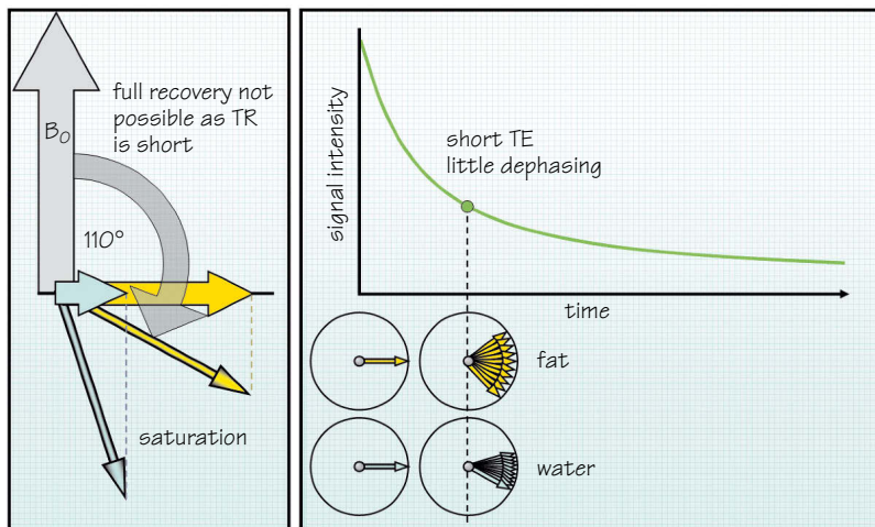
Figure 18.1 T1 weighting in gradient echo.
