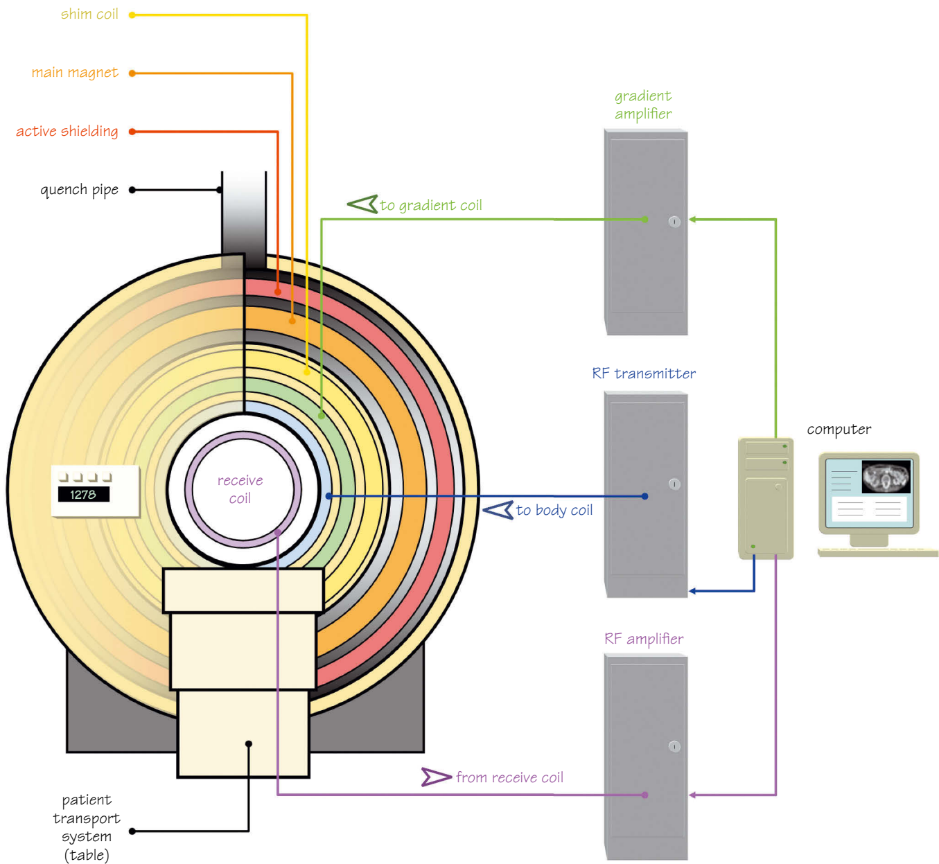
Figure 58.1 MR instrumentation.
