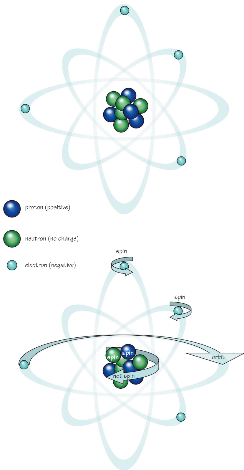
Figure 2.1 The atom.
