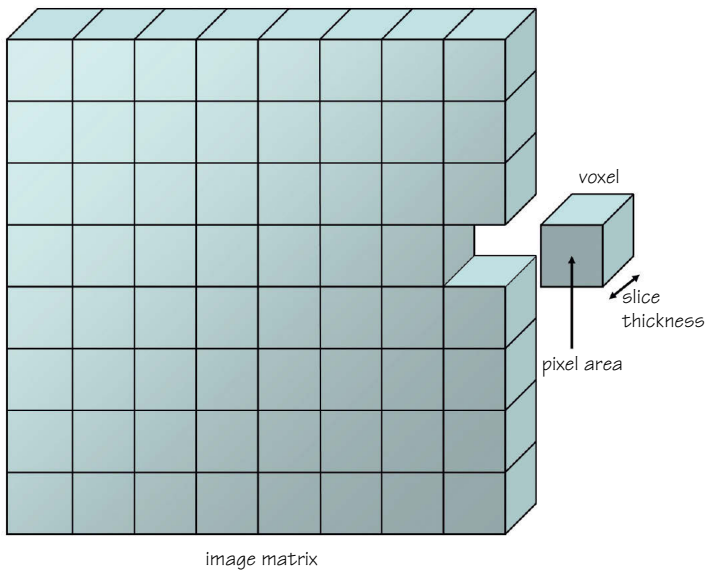
Figure 31.1 The voxel.
