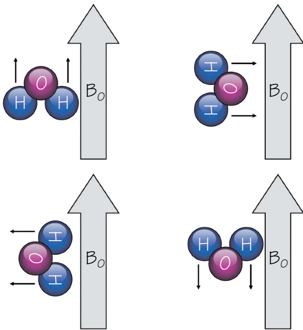
Figure 54.1 Tumbling of water molecules.
