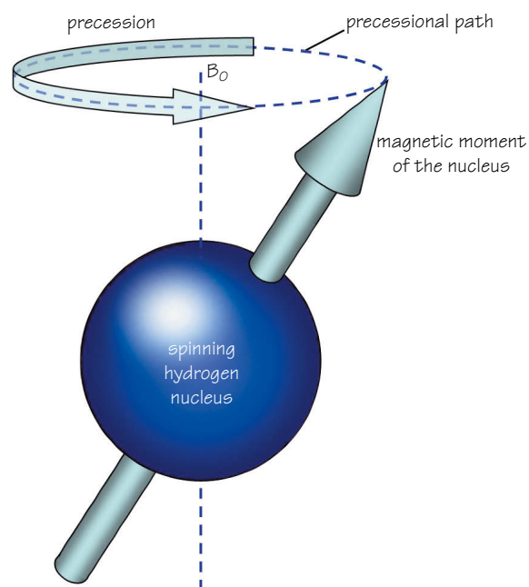
Figure 3.3 Precession.
