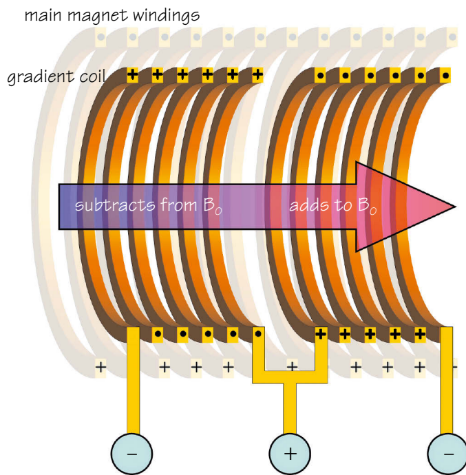
Figure 27.1 A gradient coil.
