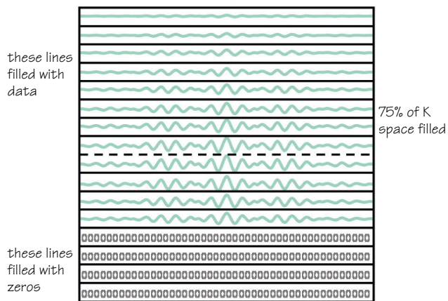
Figure 39.1 Partial Fourier.
