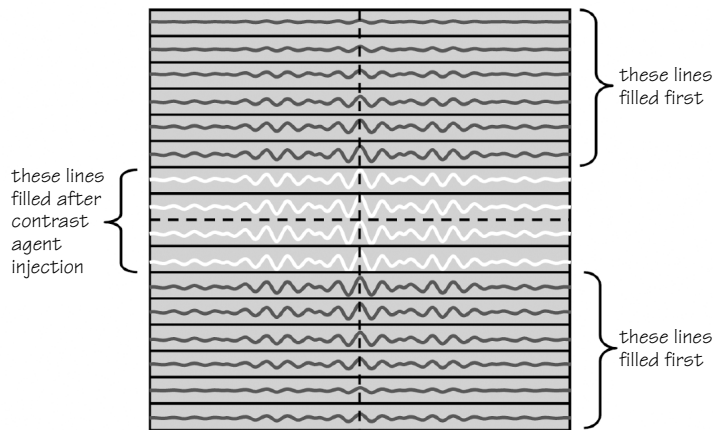
Figure 39.3 Keyhole imaging.
