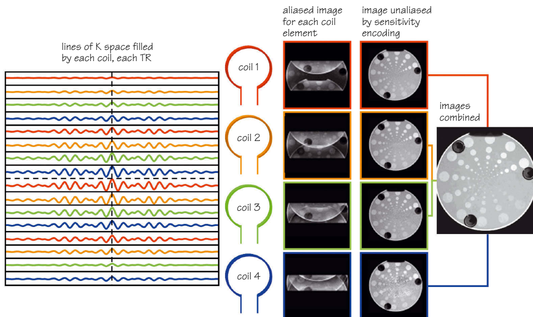
Figure 39.4 Parallel imaging.
