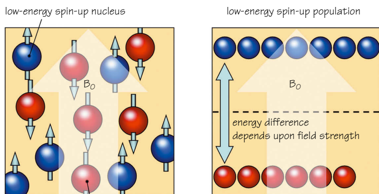
Figure 3.2 Alignment: quantum theory.
