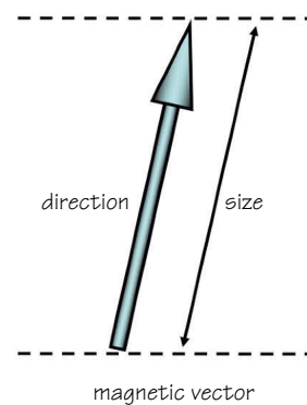
Figure 2.2 The magnetic moment of the hydrogen 1 nucleus.
