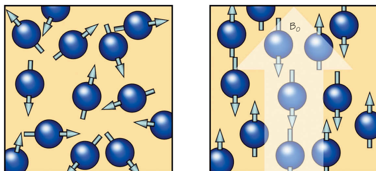
Figure 3.1 Alignment: classical theory.
