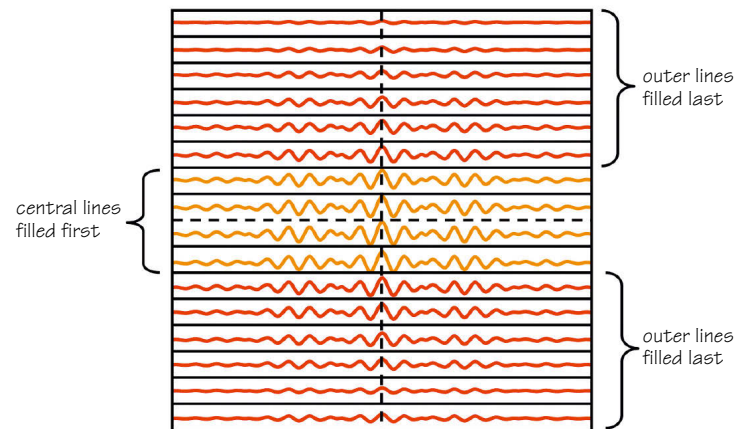
Figure 39.2 Centric K space filling.
