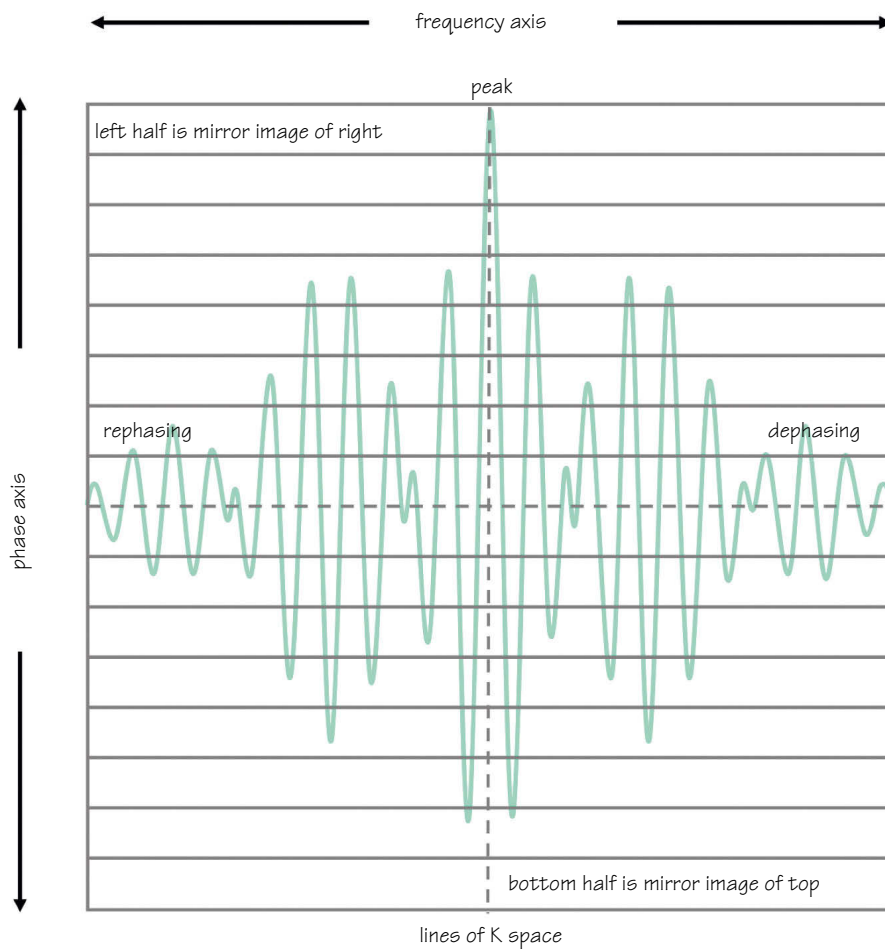
Figure 33.2 Frequency encoding vs signal amplitude.
